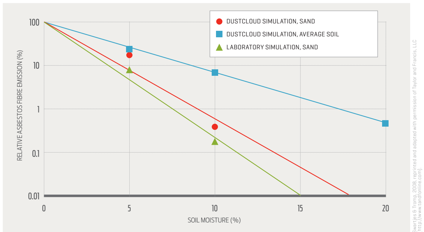
Figure 15. Asbestos fibre release in soils with differing moisture/water content.
